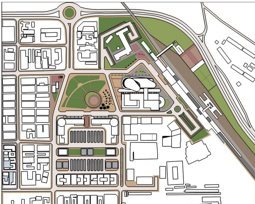
Figure 44: Proposed TOD Precinct Plan
