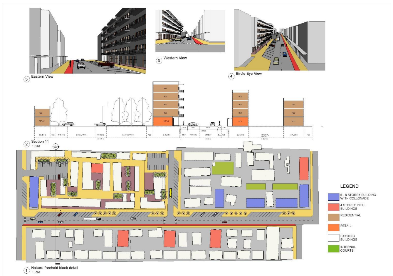
Figure 54: Proposed Intensification and Densification along Kanu Street
