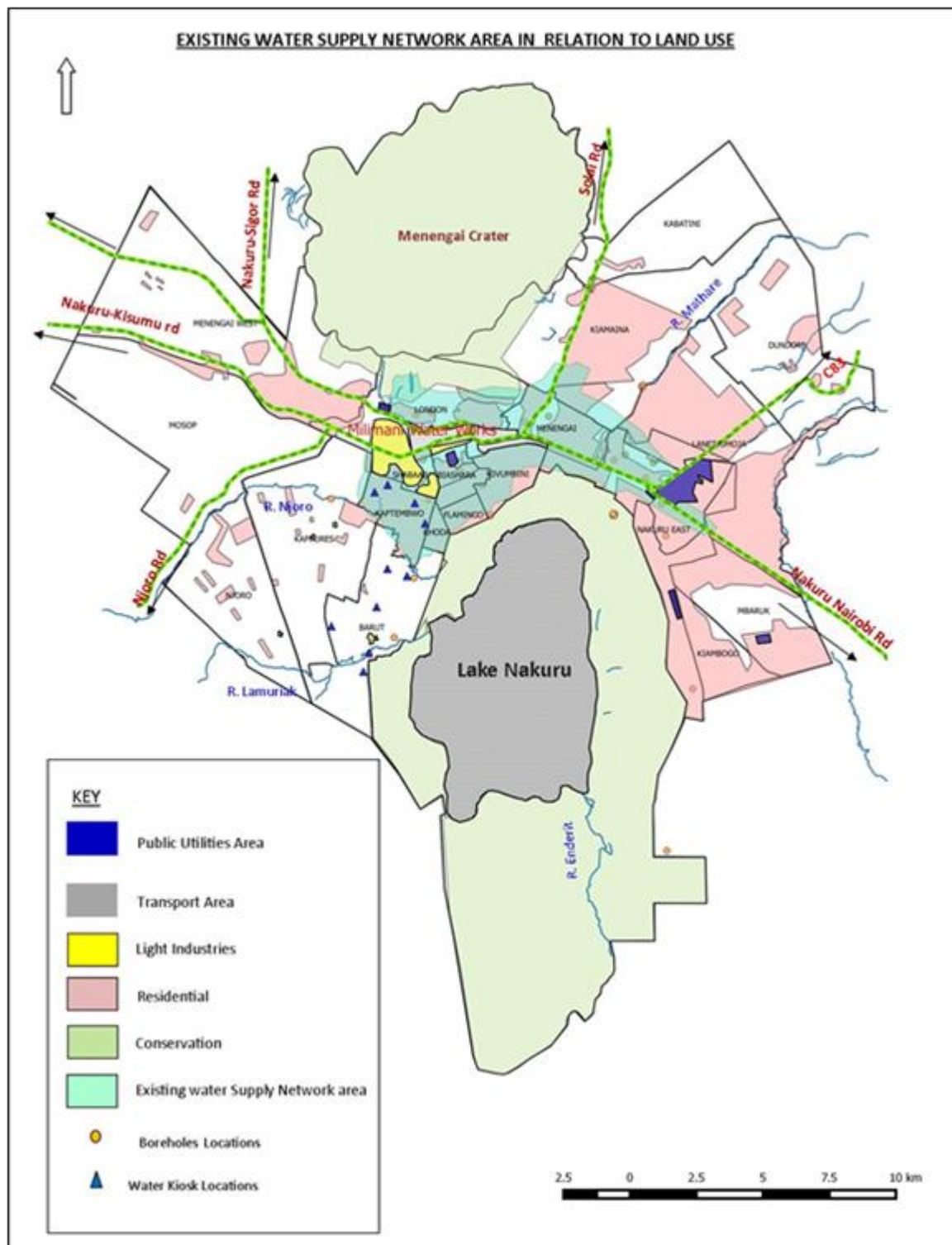
Figure 64: Existing Water Supply Network Area in Relation to Land Use
